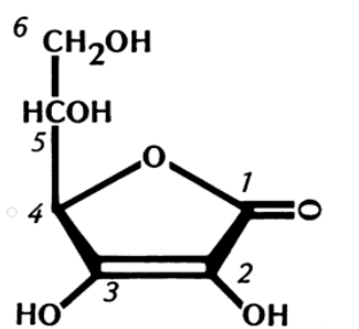
Figure 16. (a) L-ascorbic acid with numbering convention, structure is used as template in this paper with permission of the American Chemical Society (Crawford 1982); (b) Butenolide early oxidation product of L-ascorbic acid, in acidic aqueous media with \text{Cu}^{2+} oxidant, identified by John Deutsch and colleagues GCMS study (1994).
